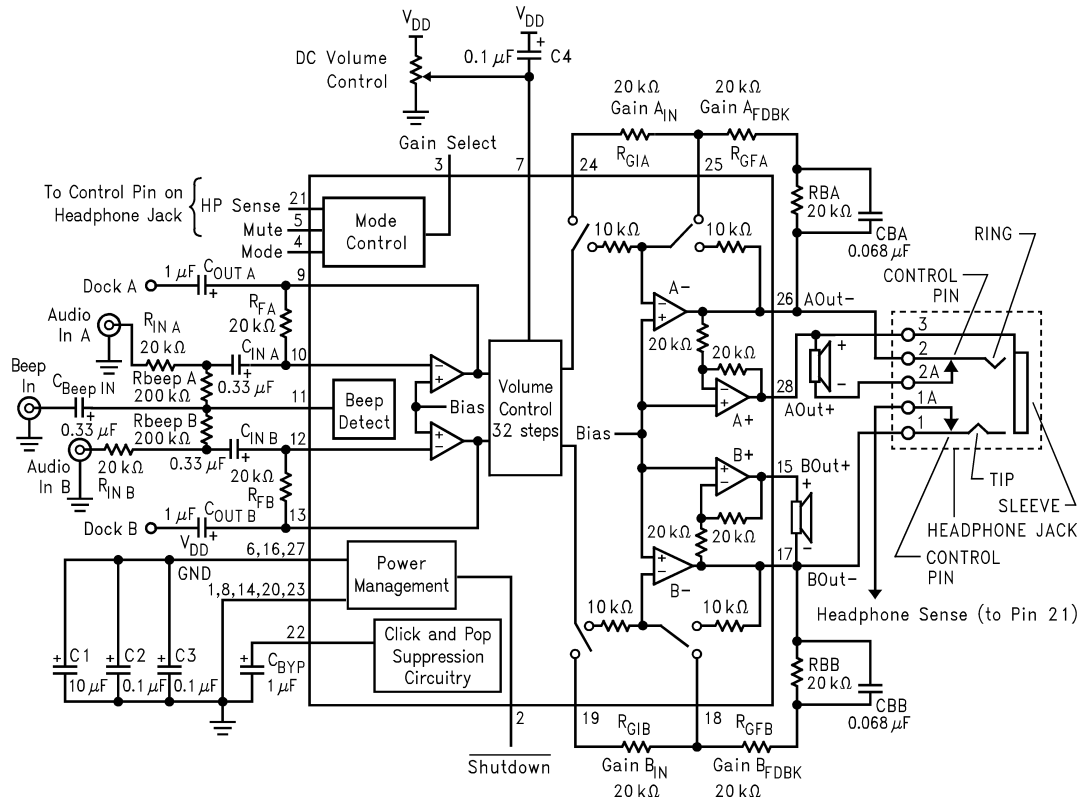
FIGURE 2. Typical Application Circuit ( MT / MH Package Pinout )
